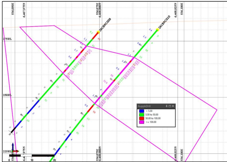
Figure 2: Cubbine Section 6468005N (Northernmost section) with Au ppb on the right and As ppm on the left. Pink outline on the left is the granite contact and the pink envelope shows the interpreted gold system.
